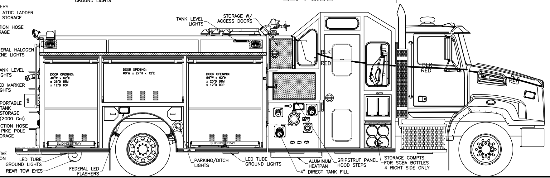
RIGHT SIDE
