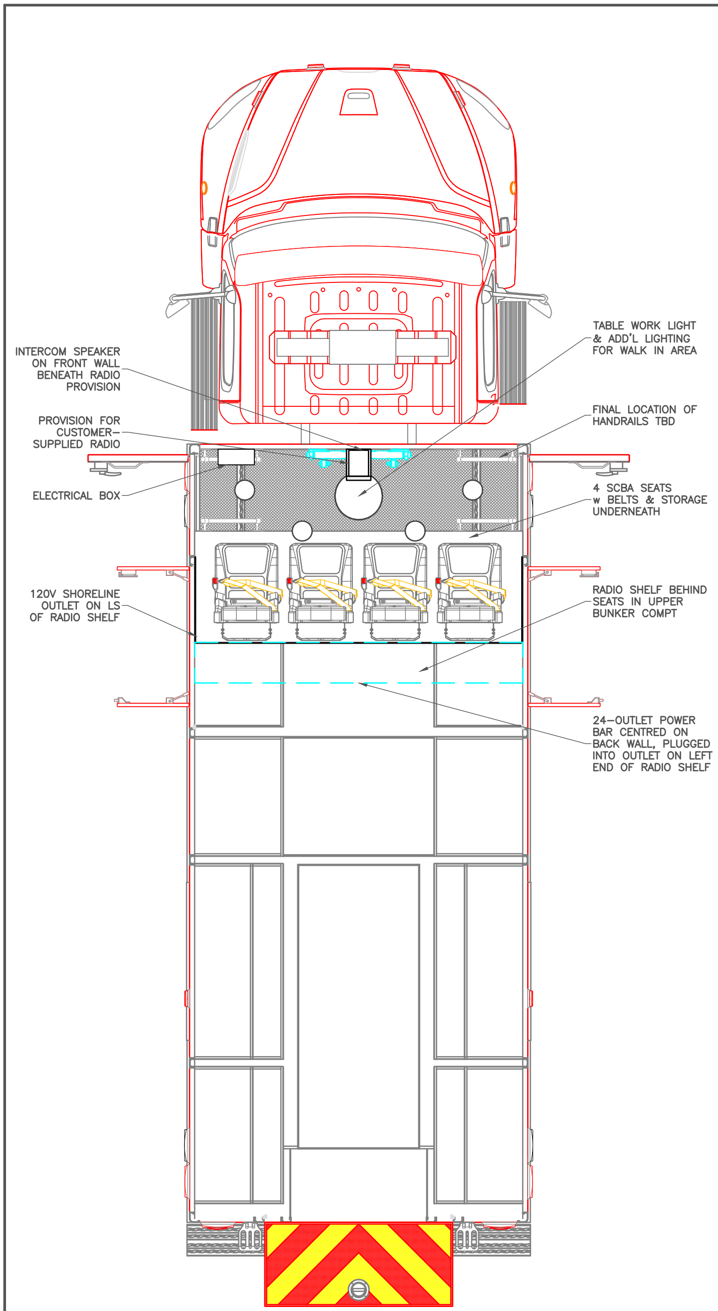
SECTION C-C
