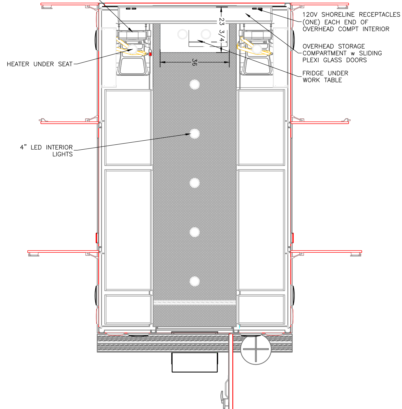
SECTION C-C
